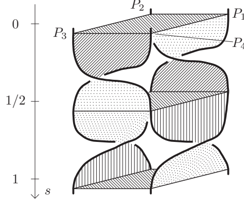
FIGURE 6. Closed braid and transverse torus
