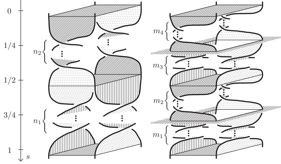
FIGURE 7. Closed braid and transverse tori for new examples
